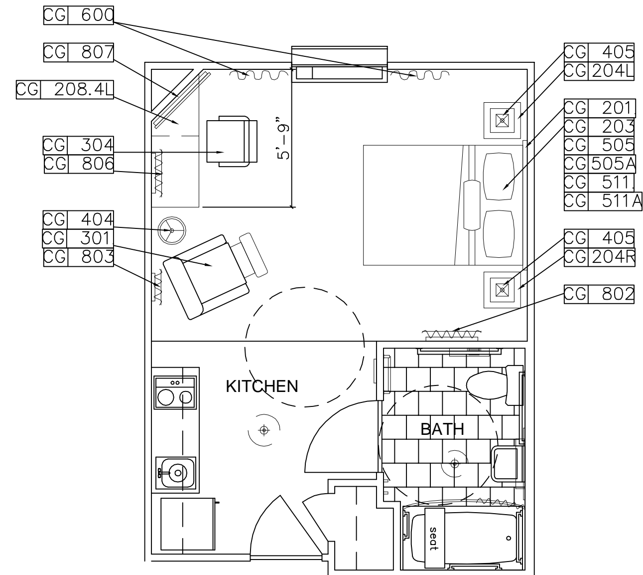
C TYPICAL ACCESSIBLE STUDIO PLAN WITH BATHTUB 1/4" = 1'-0"
