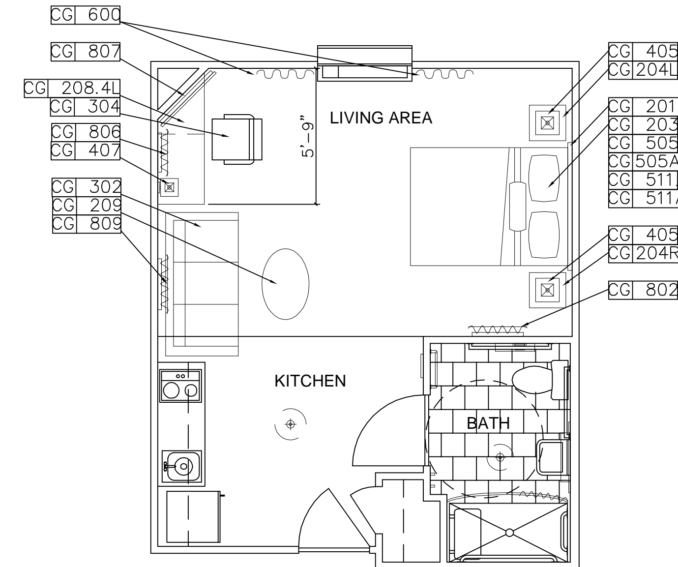
F TYPICAL ACCESSIBLE EXTENDED STUDIO PLAN QUEEN/SLEEPER SOFA OPTION WITH ROLL-IN SHOWER 1/4" = 1'-0"
