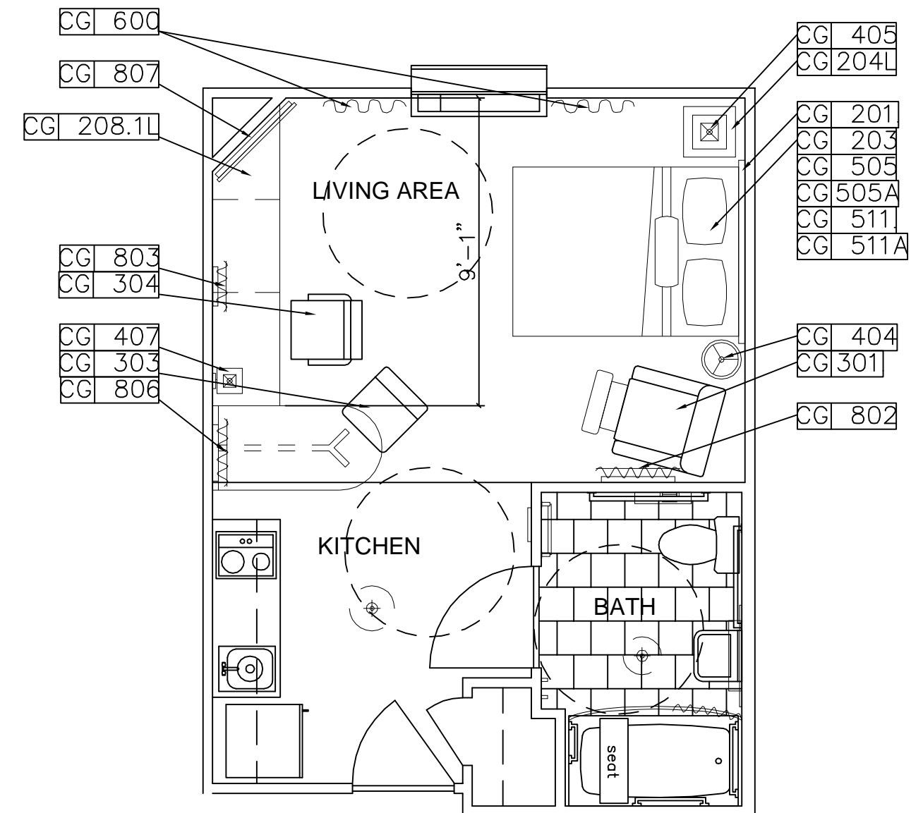
C1 TYPICAL ACCESSIBLE STUDIO PLAN WITH BATHTUB 1/4" = 1'-0"
