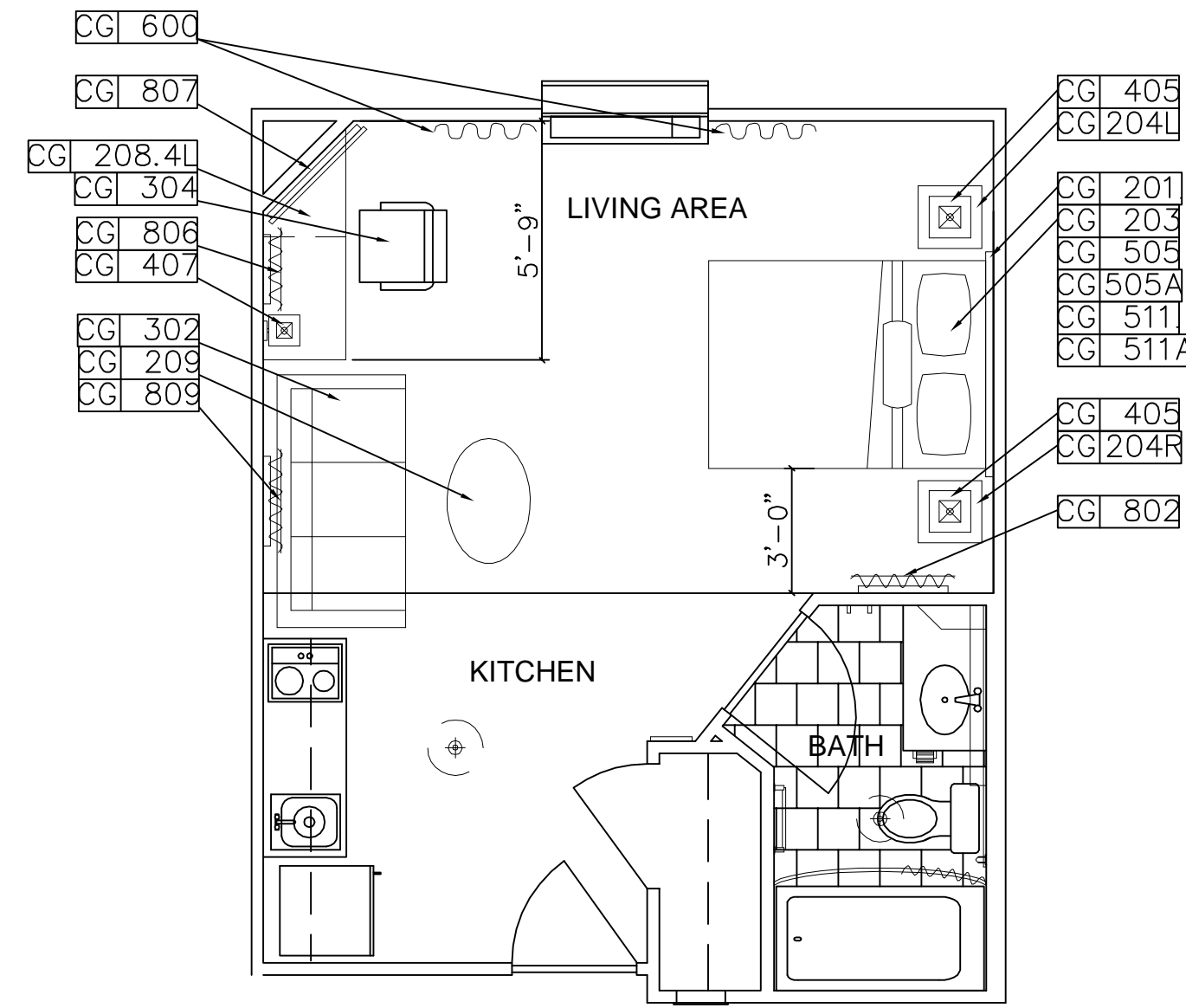
A TYPICAL EXTENDED STUDIO PLAN QUEEN/SLEEPER SOFA OPTION WITH BATHTUB 1/4" = 1'-0"
