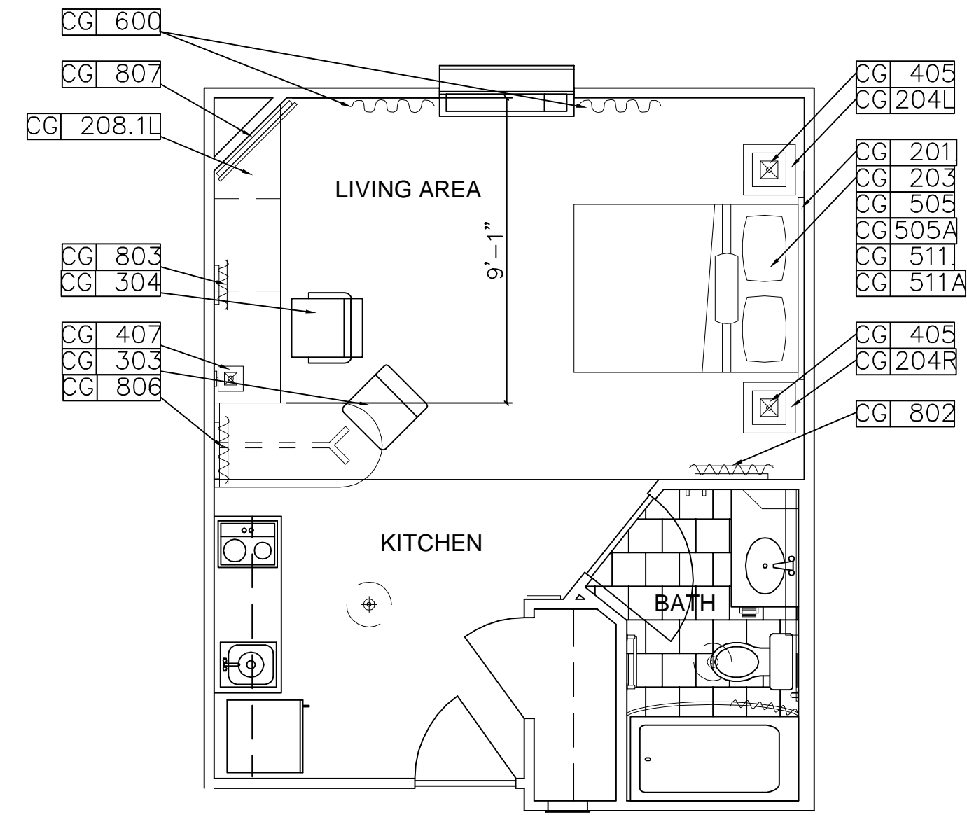
G1 TYPICAL EXTENDED STUDIO PLAN WITH BATHTUB 1/4" = 1'-0"
