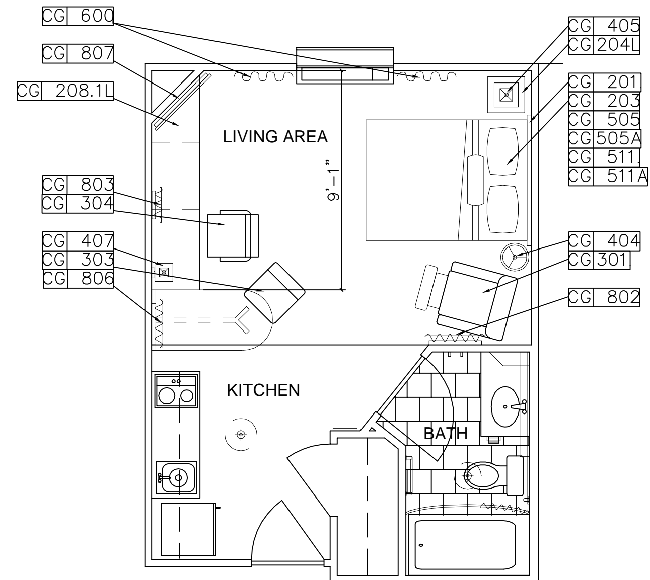
D1 TYPICAL STUDIO PLAN WITH BATHTUB 1/4" = 1'-0"
