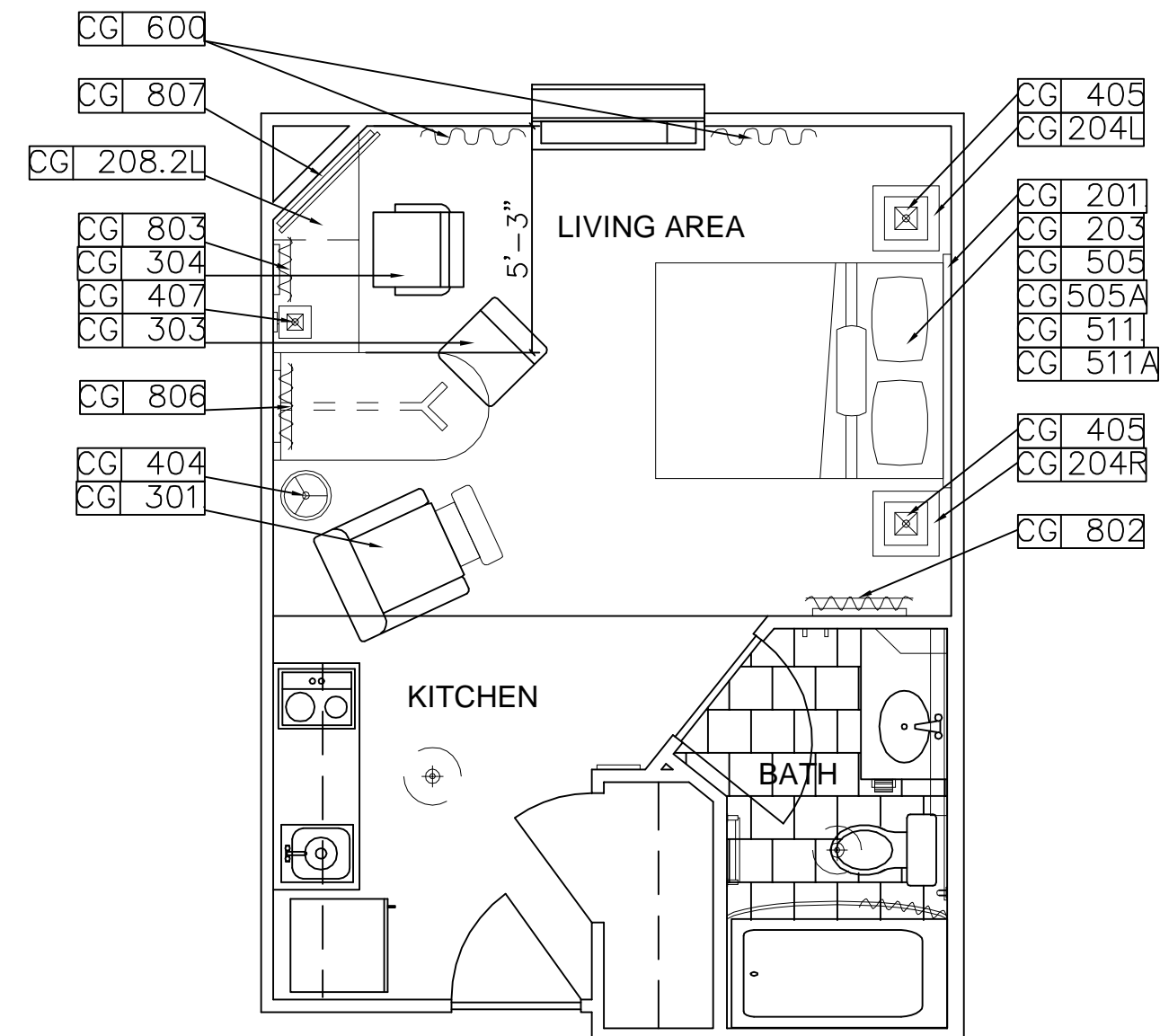
D TYPICAL STUDIO PLAN WITH BATHTUB 1/4" = 1'-0"
