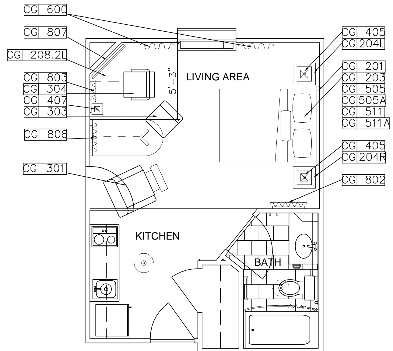
D2 TYPICAL STUDIO PLAN ADJOINING ROOMS WITH BATHTUB 1/4" = 1'-0"
