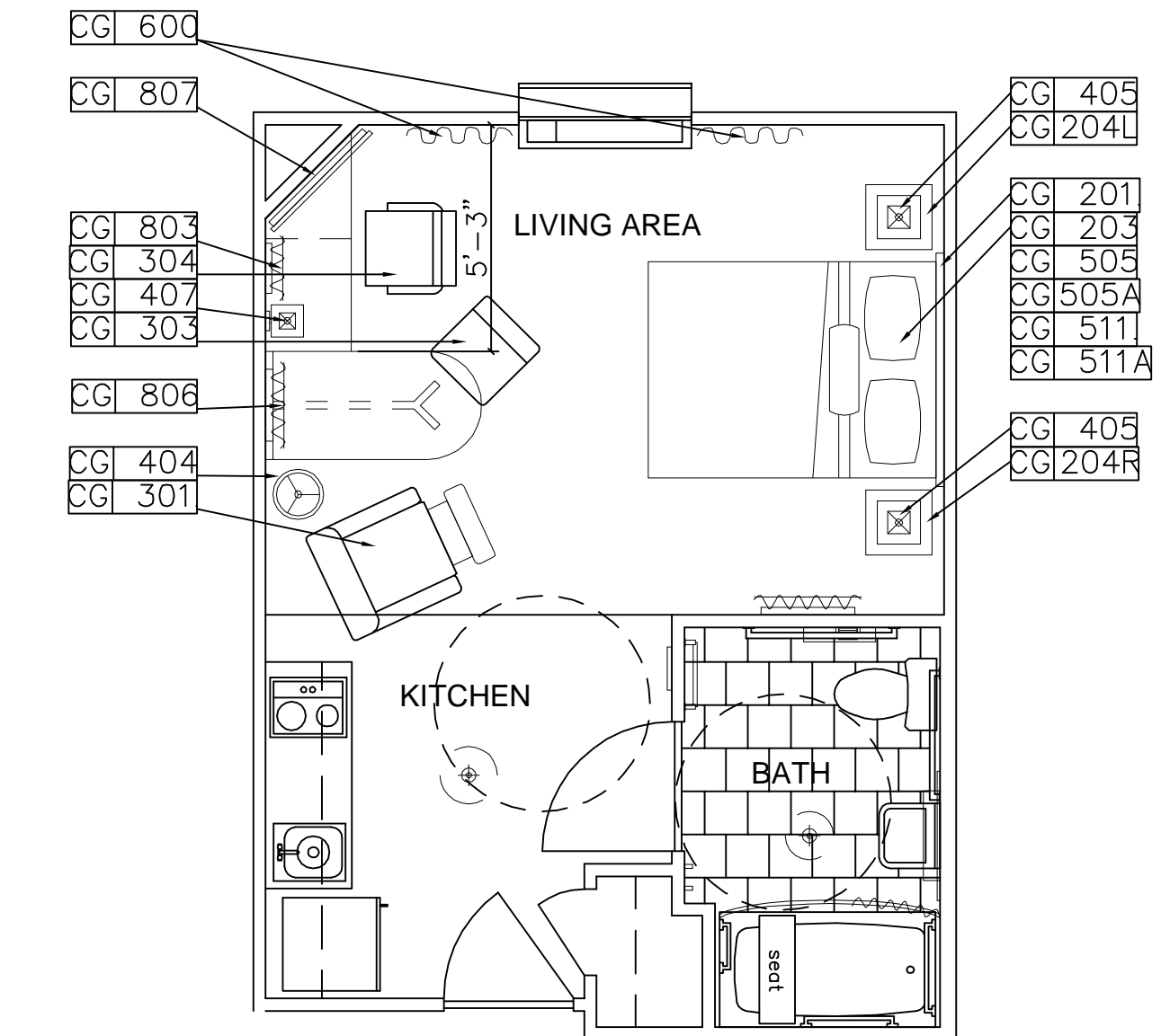
C2 TYPICAL ACCESSIBLE STUDIO PLAN WITH BATHTUB 1/4" = 1'-0"
