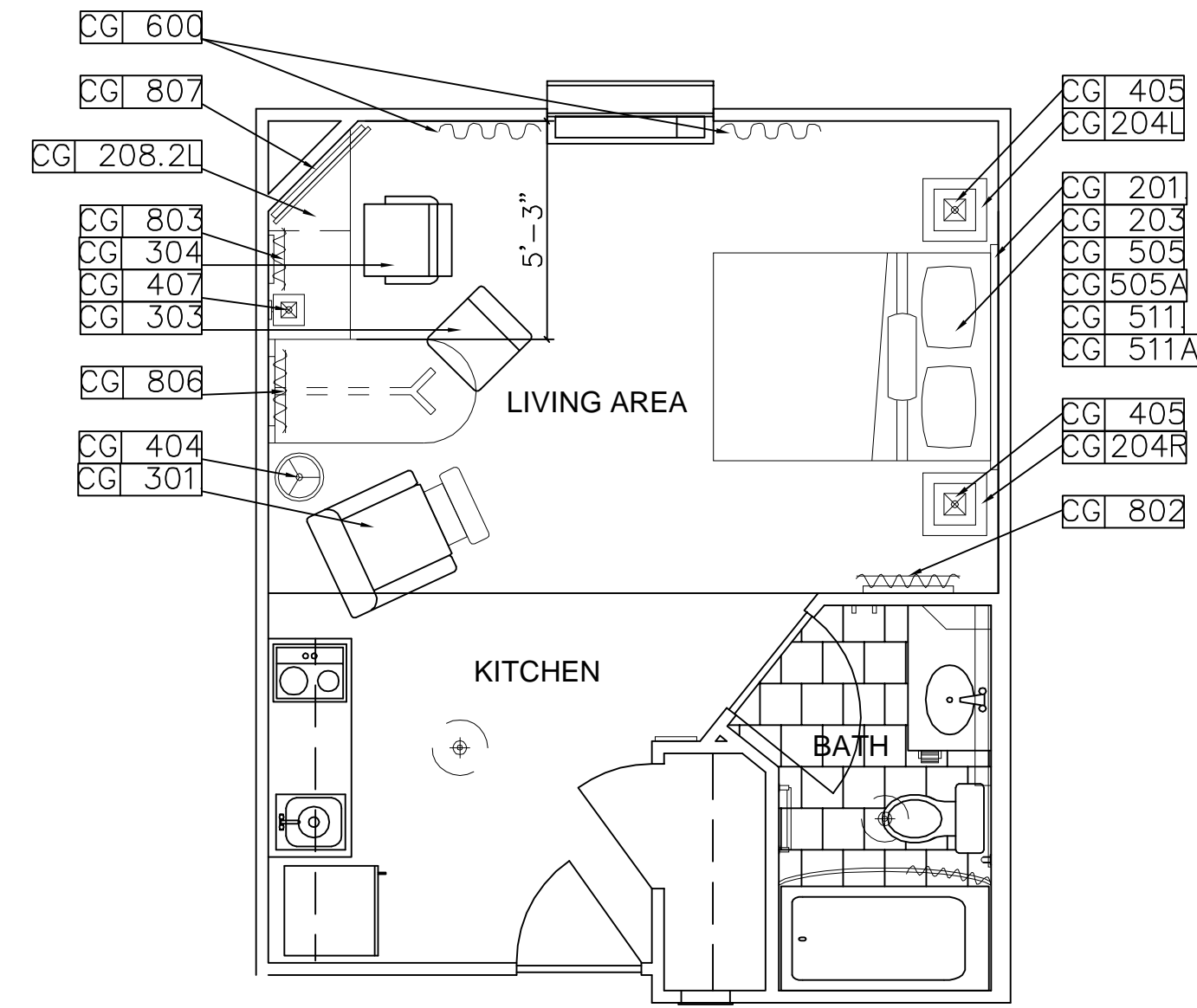
G TYPICAL EXTENDED STUDIO PLAN WITH BATHTUB 1/4" = 1'-0"
