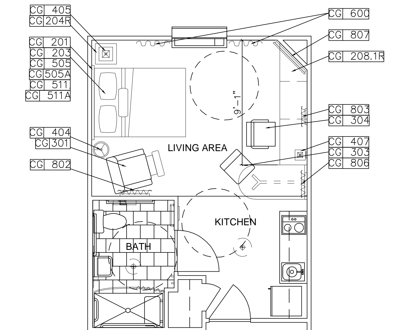
H TYPICAL ACCESSIBLE STUDIO PLAN WITH ROLL-IN SHOWER 1/4" = 1'-0"
