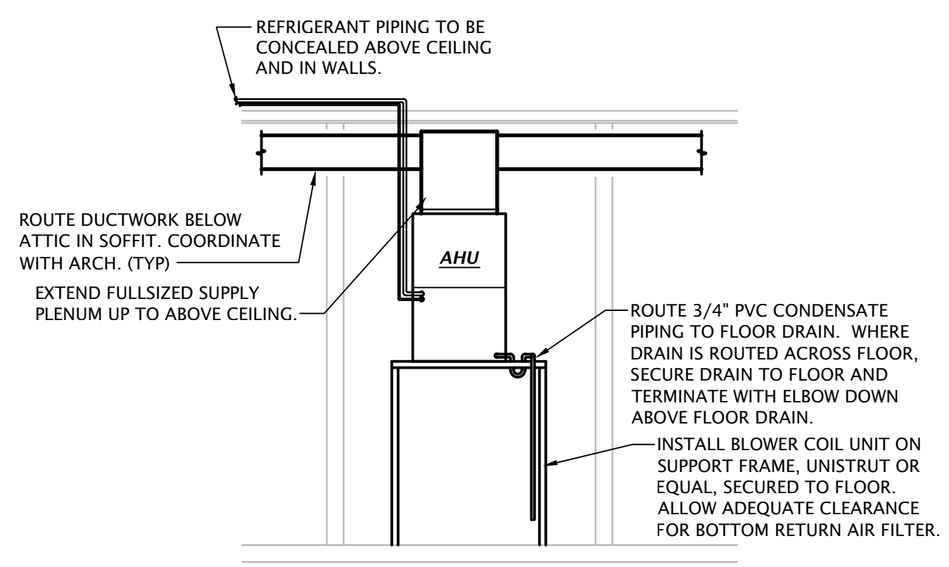
Typical AHU Detail SCALE: 1/4" = 1'-0"
